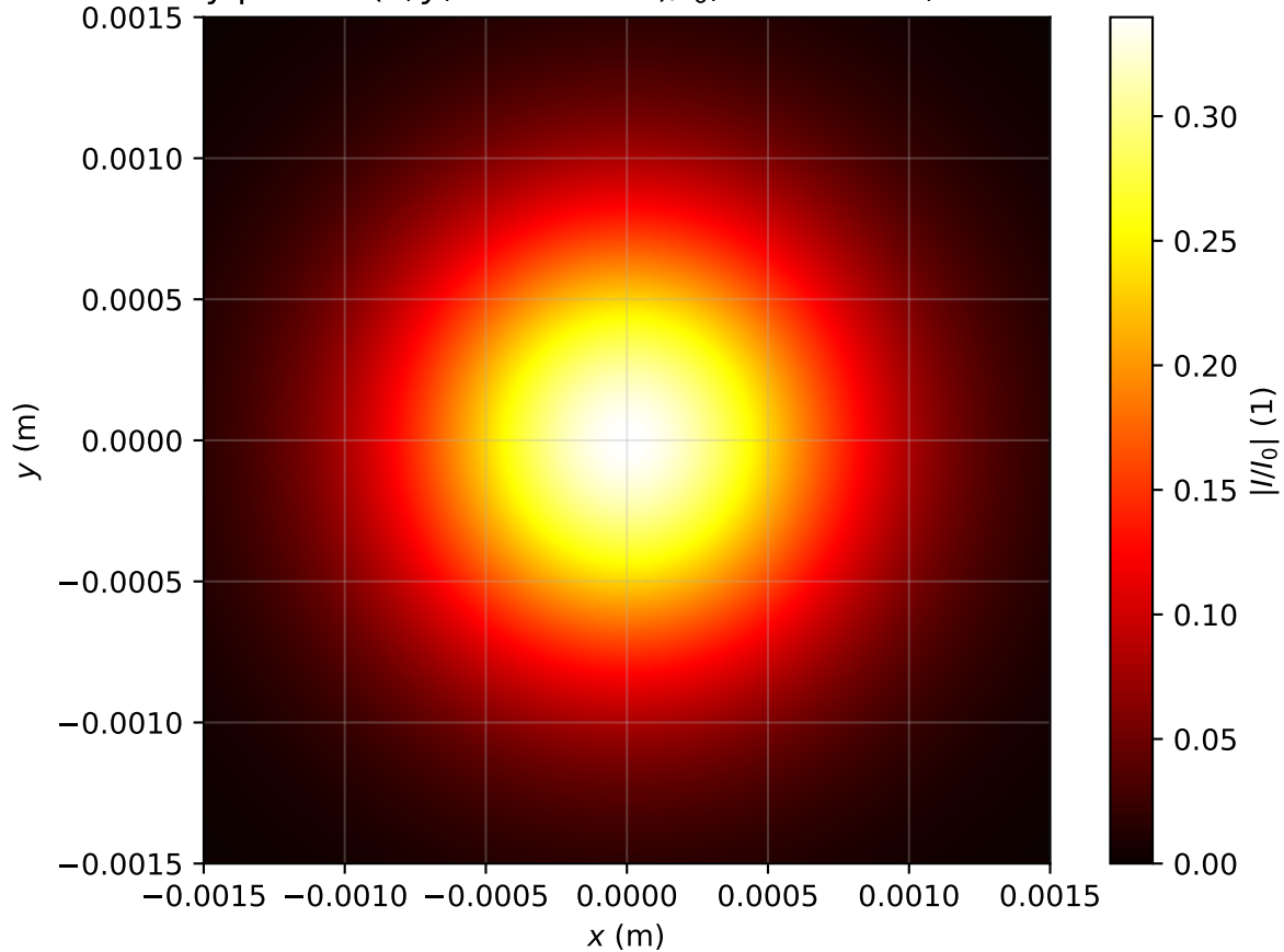
Intensity profile I(x, y, z = 3.901m)/I_0 , P_{in}=0.4P_{cr} , artificial time
